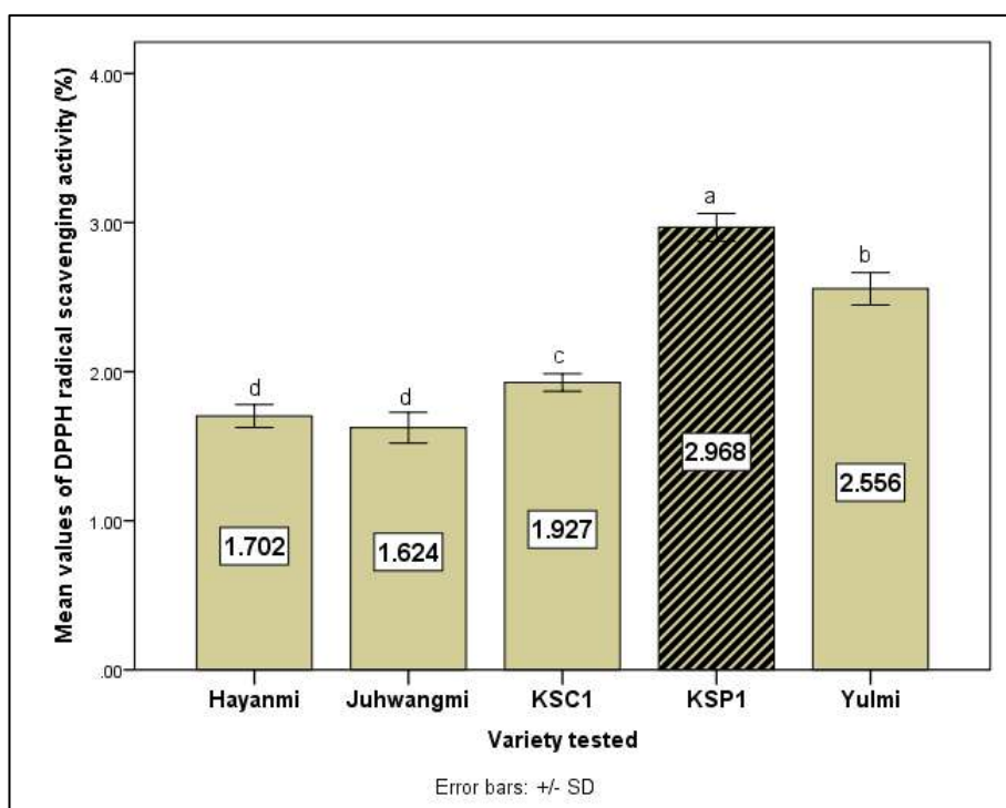
Figure 1. Antioxidant activity of sweet potato leaves by DPPH assay. Values not followed by the same letter are significantly different ( P < 0.05 ) according to Duncan's test. Abbreviations: DPPH=2, 2-diphenyl-1 picrylhydrazyl; SD=standard deviation.
