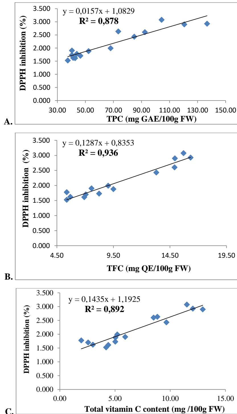
Figure 2. Relationship of total polyphenolic content (A), total flavonoid content (B) and total vitamin C content (C) with DPPH assay. Abbreviations: DPPH=2, 2-diphenyl-1-picrylhydrazyl; TPC= total polyphenol content; GAE= gallic acid equivalent; QE= quercetin equivalent; TFC= total flavonoid content.
